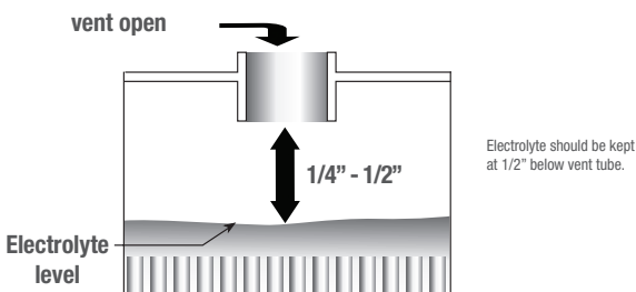
Figure 8 – Electrolyte level
