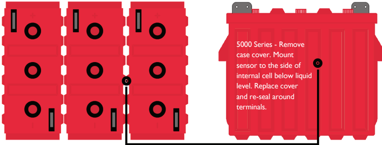
Figure 7 – Temperature Probe
