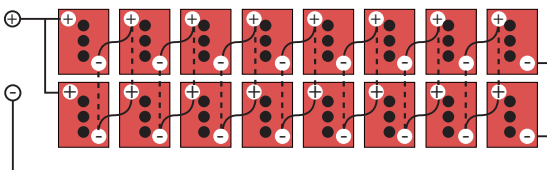
Figure 6 Two Parallel Strings. Series/Parallel with cross tie connections
